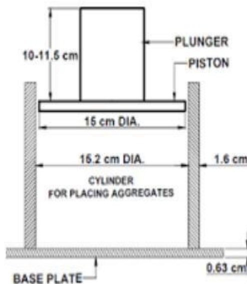
Fig. Arrangement of Crushing strength test
